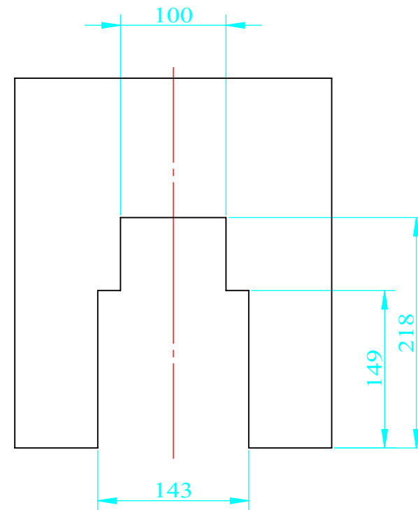
Hole dimension
